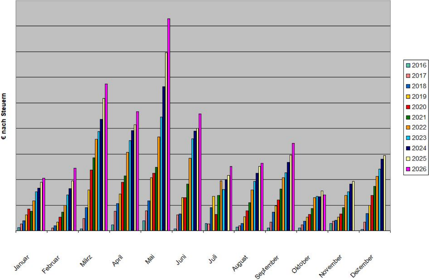
Dividenden 2016 vs 2017 vs 2018 vs 2019 vs 2020 vs 2021 vs 2022 vs 2023 vs 2024 vs 2025 vs 2026
